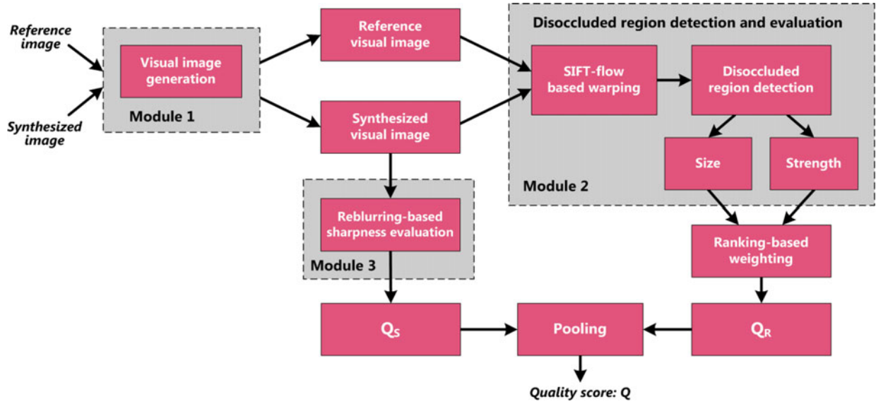
Fig. 2. Flowchart illustration of the proposed quality model for DIBR-synthesized images.
